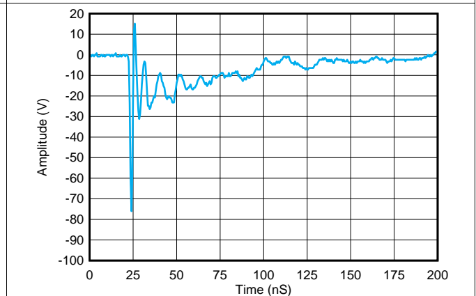
Figure 6. IEC Clamping Waveforms (-8-kV Contact)
