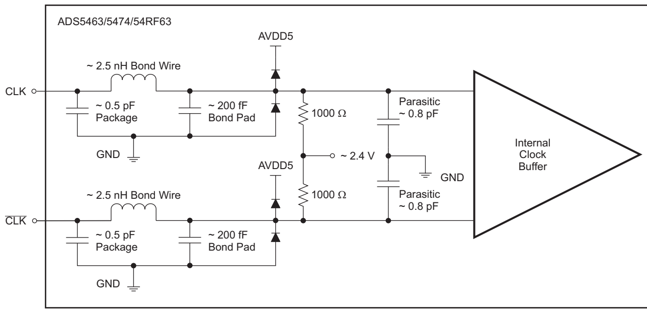
Figure 57. Clock Input Circuit (unsoldered package)
