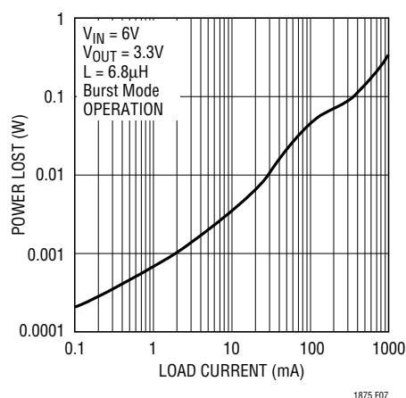
Figure 7. Power Lost vs Load Current
