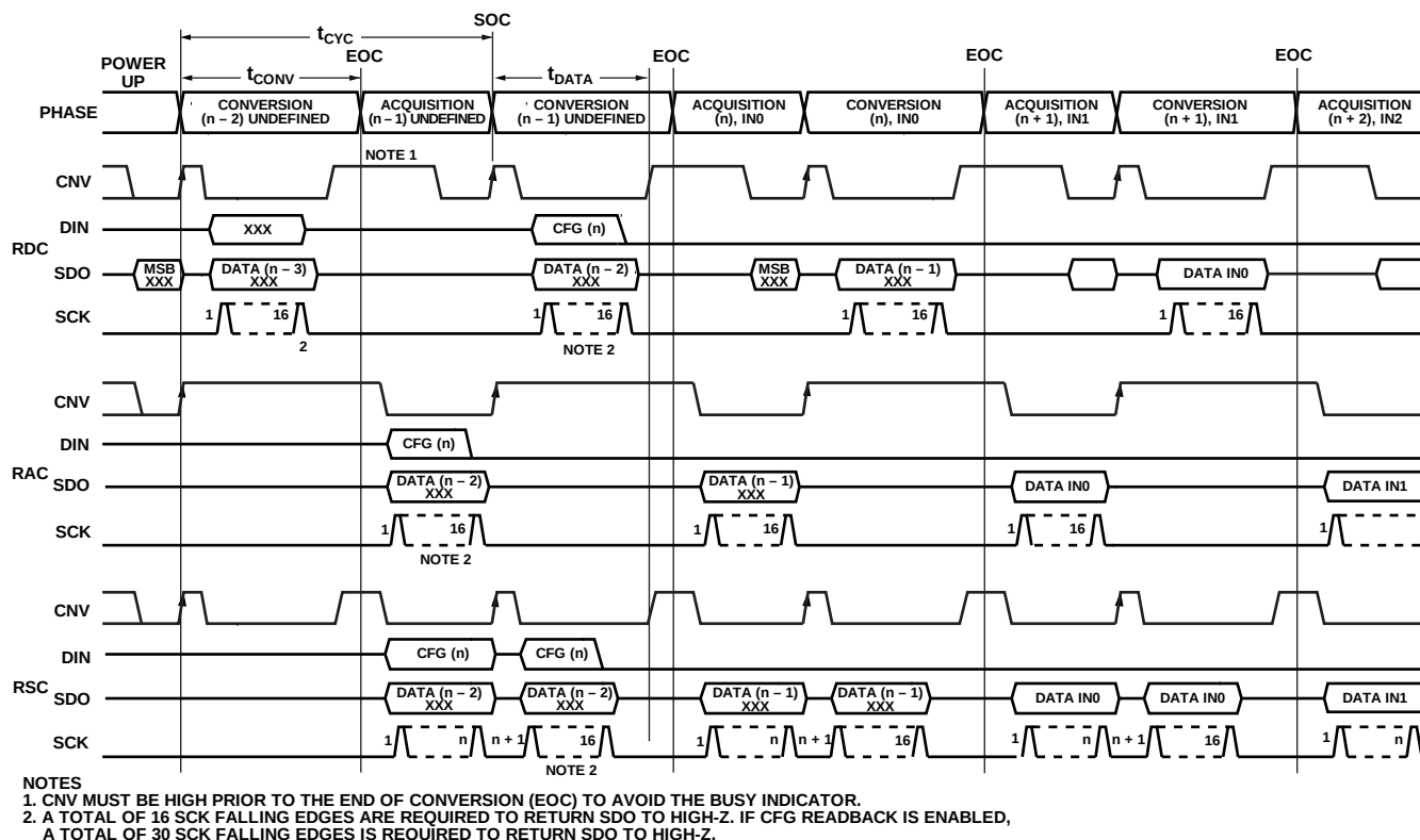
Figure 43. General Channel Sequencer Timing Without a Busy Indicator
