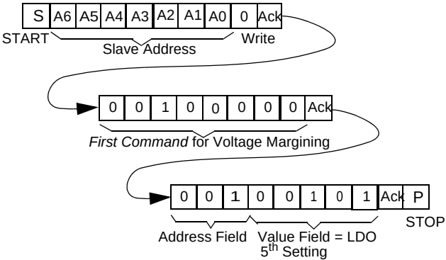
Figure 26. Complete Data Transfer Example
