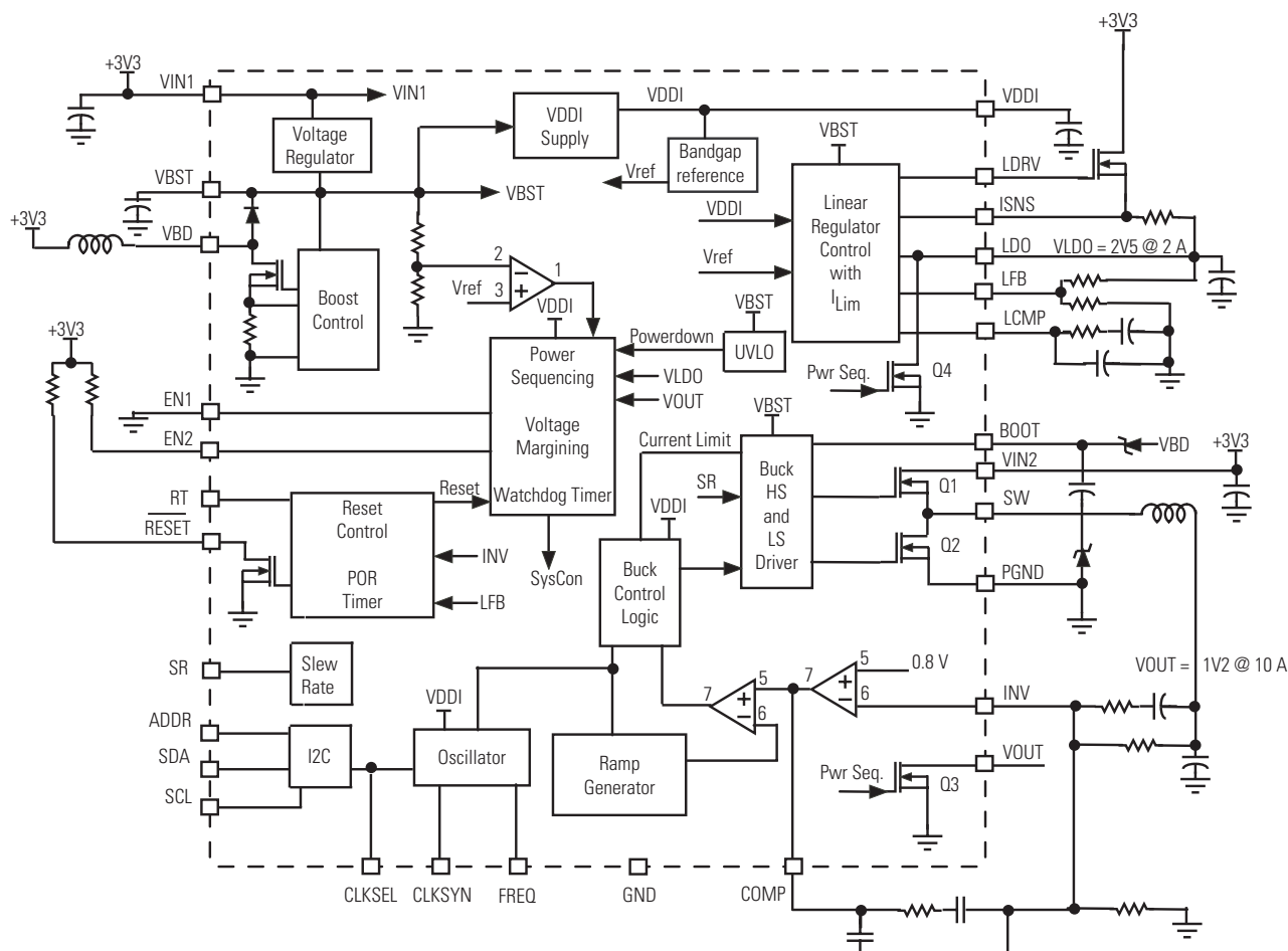
Figure 27. 34703 Typical Application
