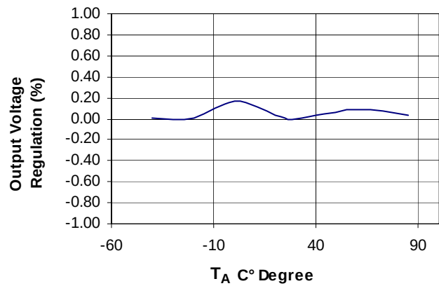
Figure 8. Buck Converter Voltage Regulation vs Ambient Temperature
