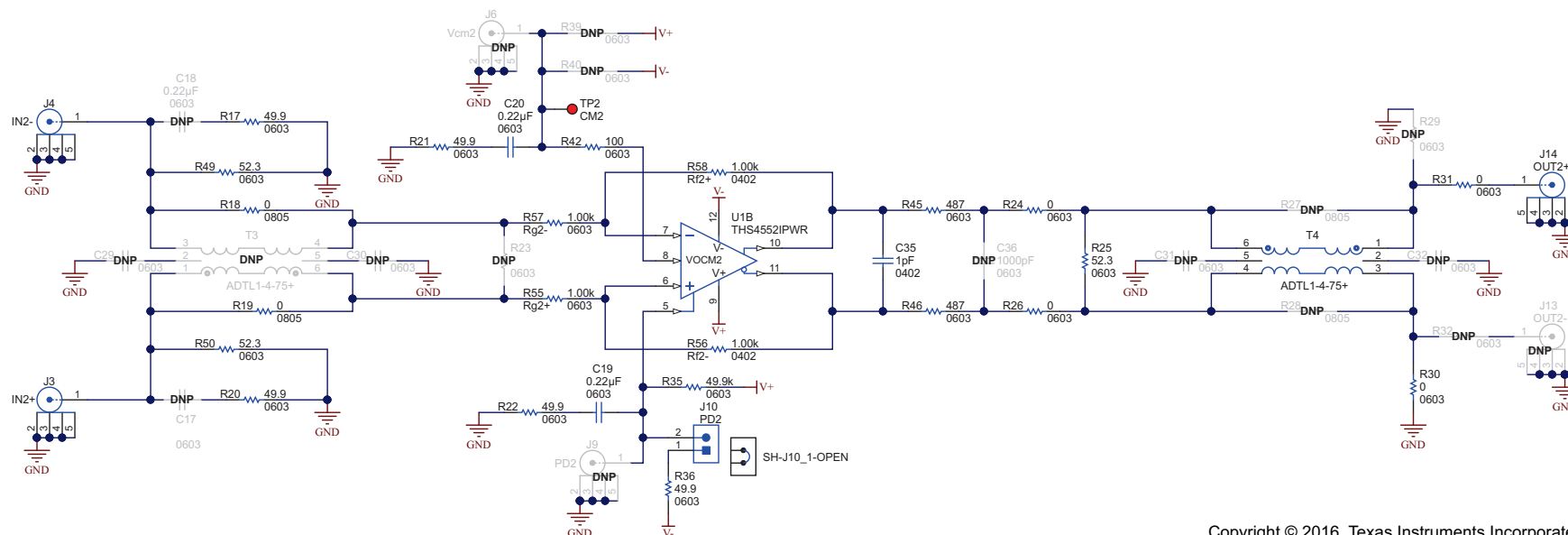
Figure 2. THS4552PWEVM Schematic
