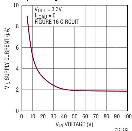
V_{IN} Input Current in Regulation vs Input Voltage
