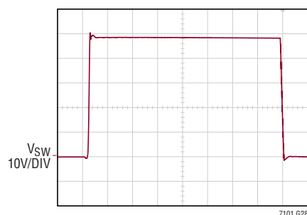
SW Node Waveform at Full Load
