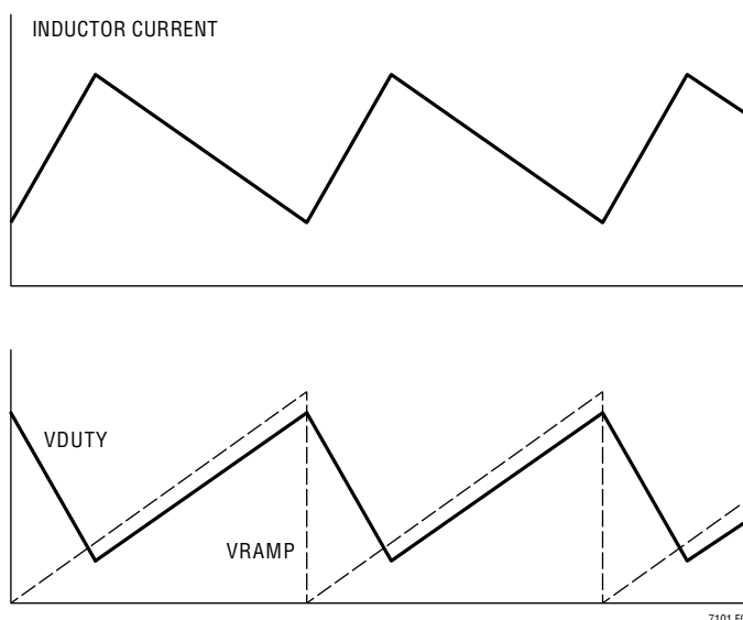
Figure 1. Typical Current Loop Operating Waveforms
