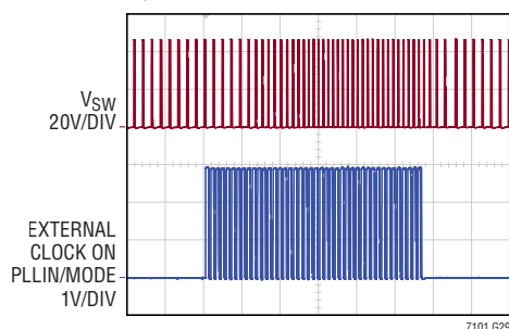
Synchronization to External Clock
