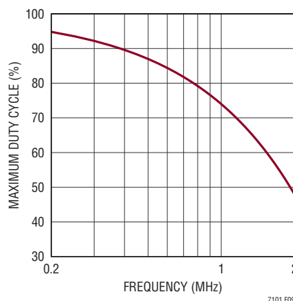
Figure 9. Maximum Allowable Duty Cycle vs Frequency for V_{OUT} > 6V and Option 2 Configuration
