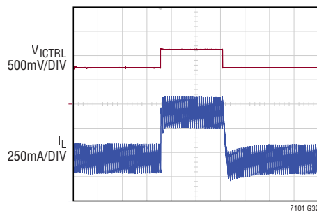
Output Current Programming Current Loop Step Response
