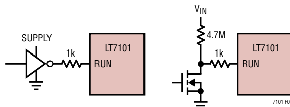
Figure 7. RUN Pin Interface to Logic
