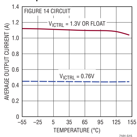
Average Output Current vs Temperature
