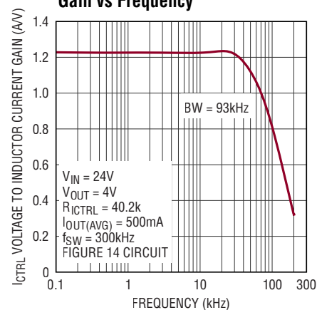
ICTRL Voltage to Inductor Current Gain vs Frequency
