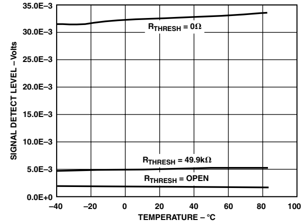
TPC 2. Signal Detect Level vs. Temperature
