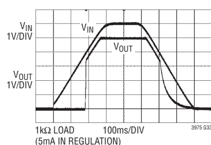
Start-Up/Dropout Performance
