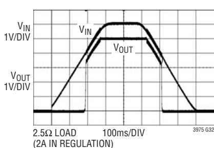
Start-Up/Dropout Performance
