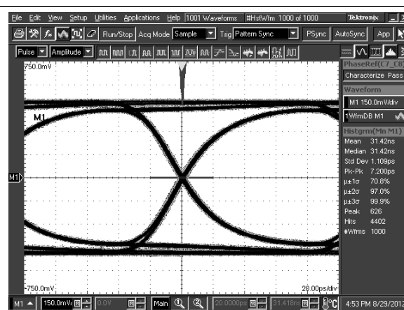
DS125BR800 settings: EQ[1:0] = 0, F = 0x02, DEM[1:0] = 0, 1 Figure 13. TL = 10 inch 5-mil FR4 trace, 8 Gbps
