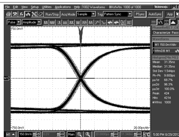
DS125BR800 settings: EQ[1:0] = 0, 1 = 0x03, DEM[1:0] = 0, 1 Figure 15. TL = 20 inch 5-mil FR4 trace, 5 Gbps
