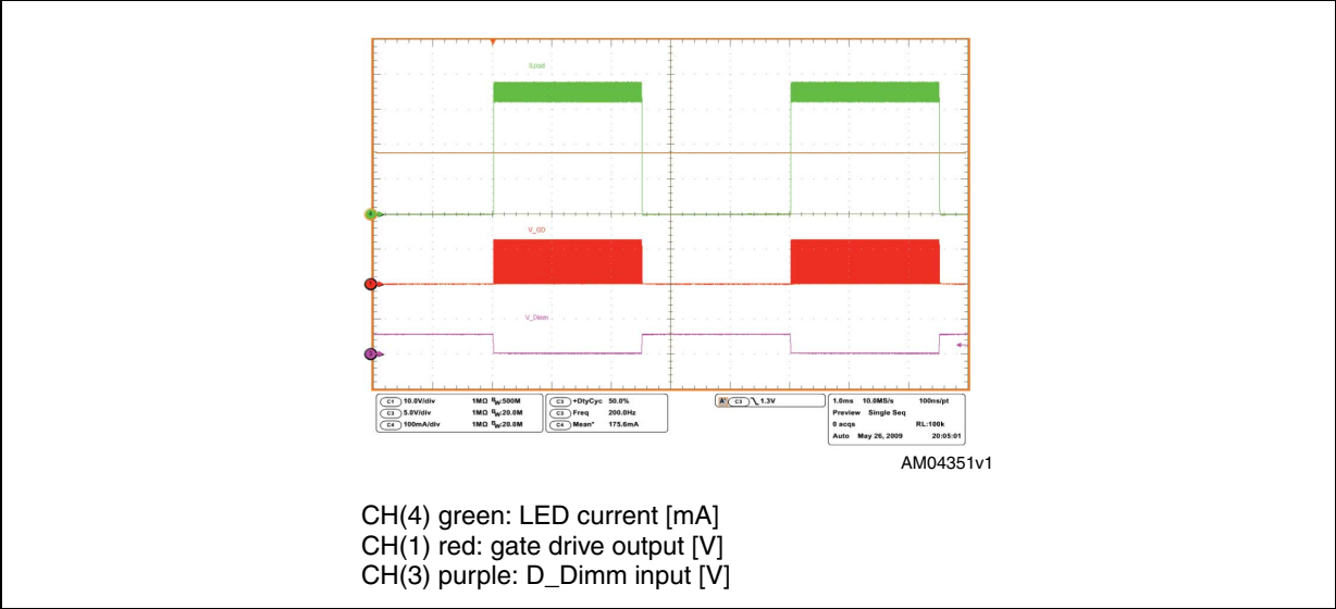
Figure 18. Dimming 50%
