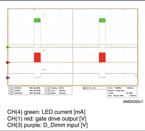
Figure 17. Dimming 10%
