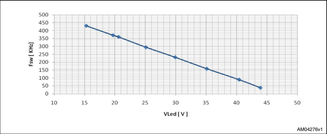
Figure 29. Switching frequency
