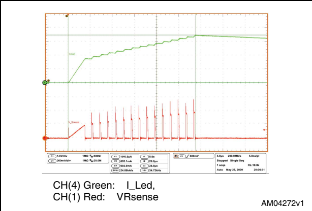
Figure 25. Short-circuit detection
