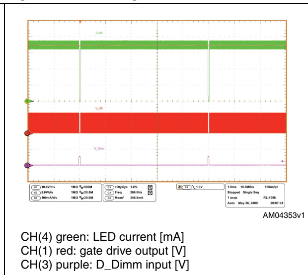
Figure 20. Dimming 99%
