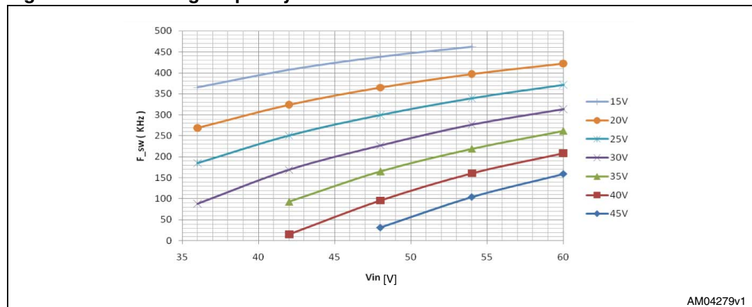
Figure 32. Switching frequency
