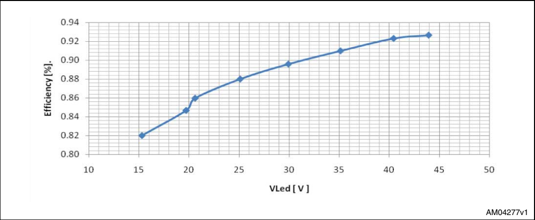
Figure 30. Efficiency [%]
