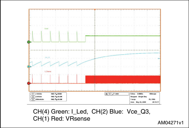
Figure 24. Short-circuit removal
