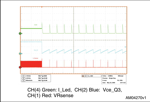
Figure 23. Short-circuit application
