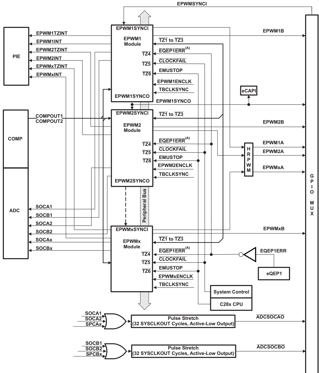
Figure 6-48. ePWM
