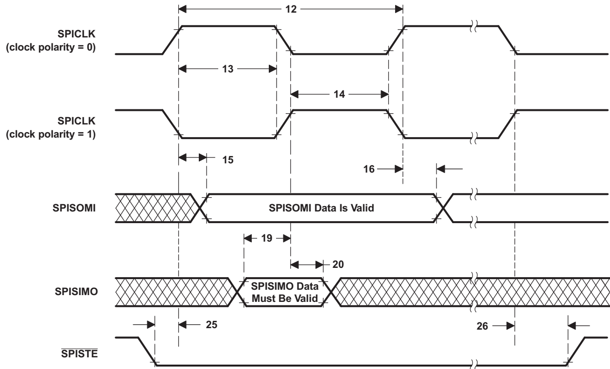
Figure 6-35. SPI Slave Mode External Timing (Clock Phase = 0)
