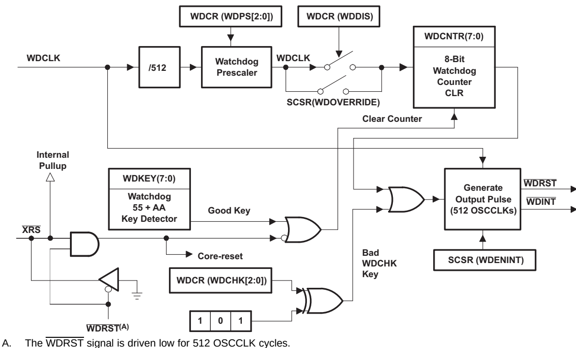
Figure 6-15. CPU Watchdog Module
