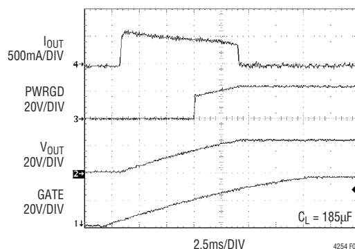
Figure 6. Start-Up Waveforms
