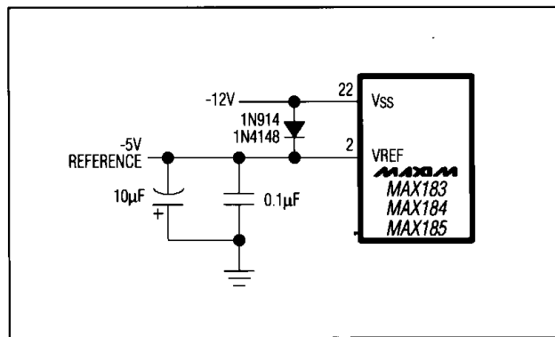
Figure 12. VREF/VSS Diode Clamp (See "Reference Input" Text).
