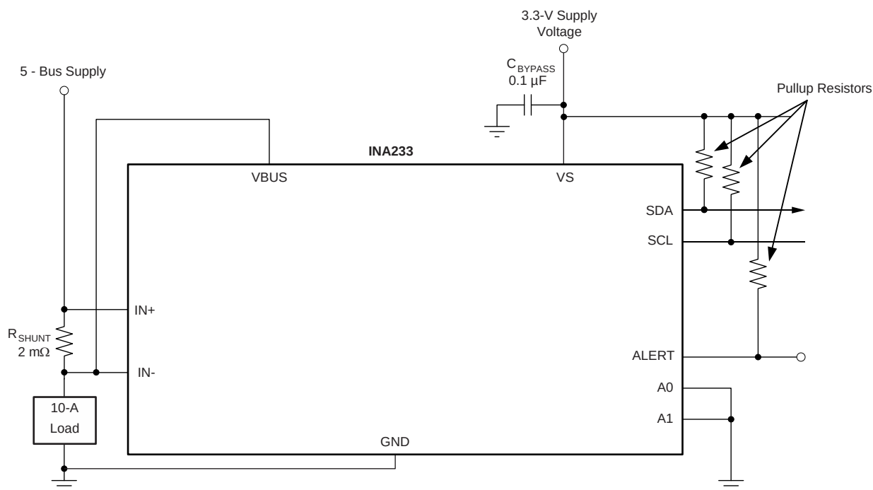
Figure 43. Typical High-Side Sensing Circuit Configuration, INA233
