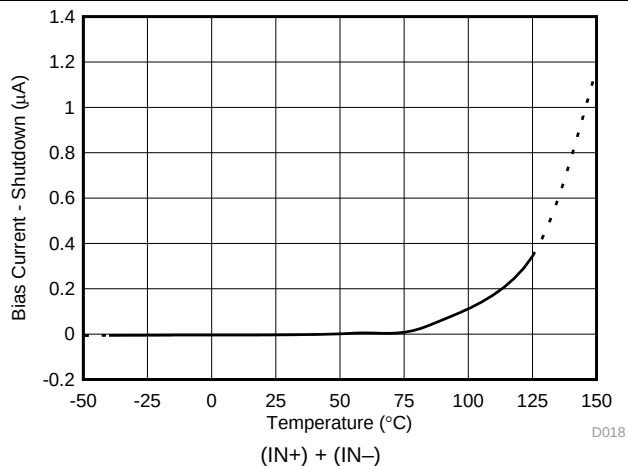
Figure 18. Input Bias Shutdown Current vs Temperature
