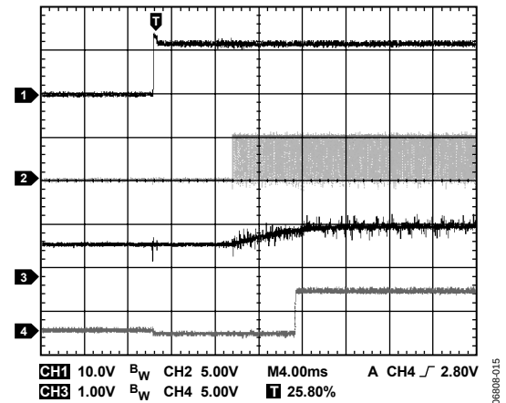
Figure 15. Start into Precharged Channel 2 Channel 1: V IN , Channel 2: Low-Side Gate, Channel 3: V OUT2 , Channel 4: POK
