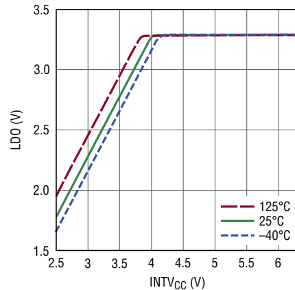
LD033 Pin Regulation ( I_{LD033} = 1\text{mA} )
