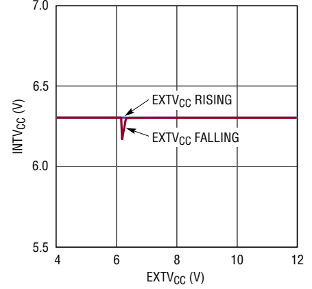
INTV CC Line Regulation ( V_{IN} = 12\text{V} )
