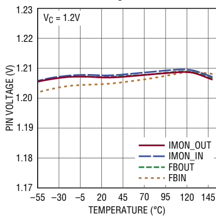
Feedback Voltages
