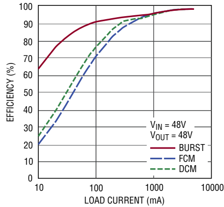
Efficiency vs Output Current (Buck-Boost Region-Figure 15)
