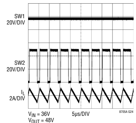
Forced Continuous Mode (Figure 15)
