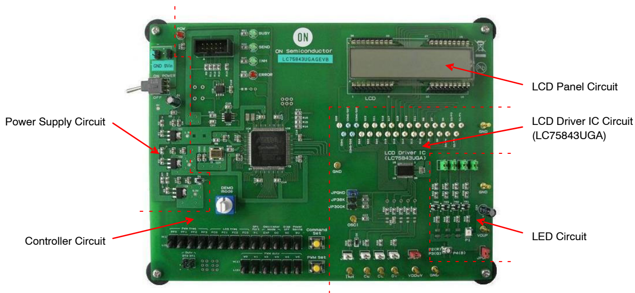
Figure 1. Appearance of LCD Driver IC Evaluation Board (LC75843UGAGEVB)
