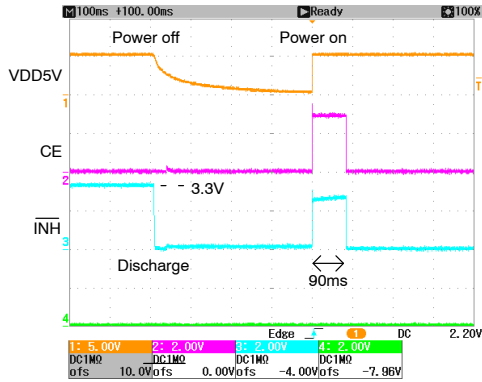
Figure 16. \overline{\text{INH}} Signal Pulse Just After the Power Supply (FPGA Output)
