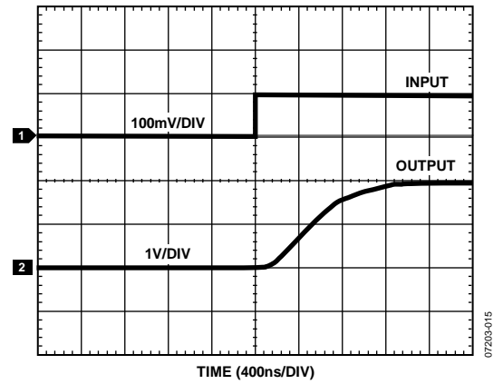
Figure 14. Rise Time
