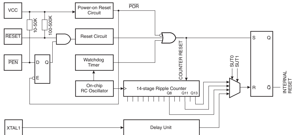
Figure 23. Reset Logic
