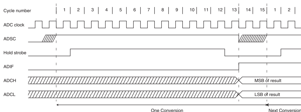
Figure 48. ADC Timing Diagram
