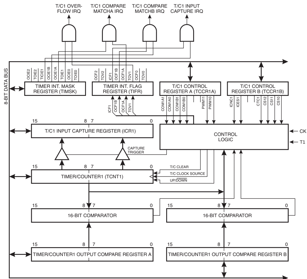
Figure 33. Timer/Counter1 Block Diagram
