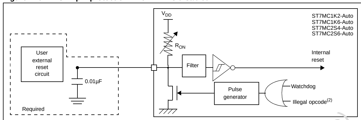
Figure 146. RESET pin protection when LVD is disabled (1)
