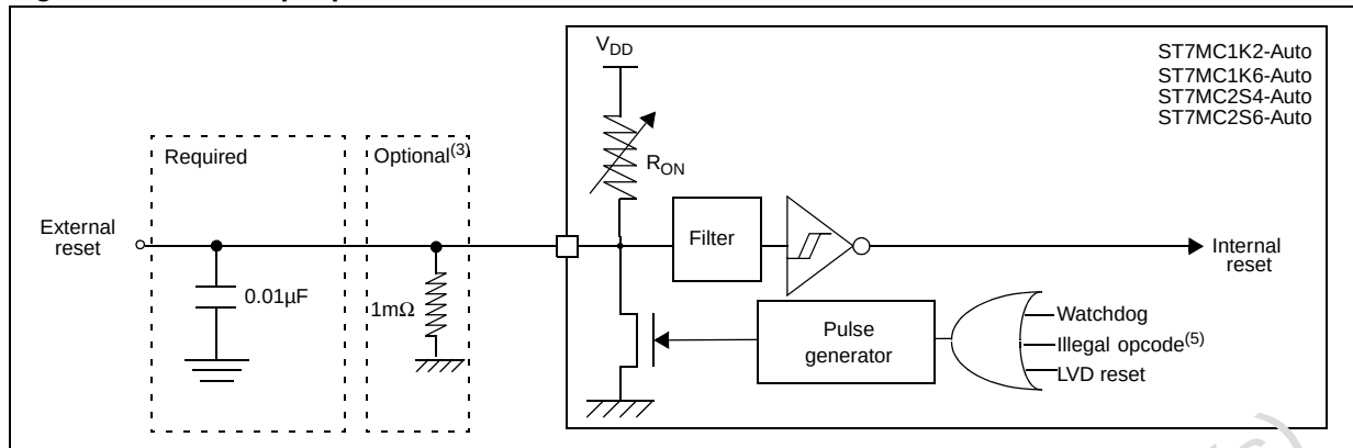
Figure 145. RESET pin protection when LVD is enabled (1)(2)(4)
