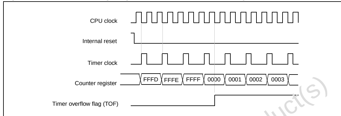
Figure 42. Counter timing diagram, internal clock divided by 2
