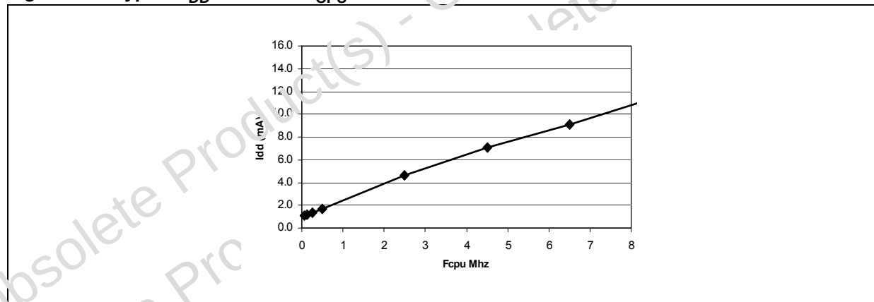
Figure 132. Typical I_{DD} in RUN vs f_{CPU}
