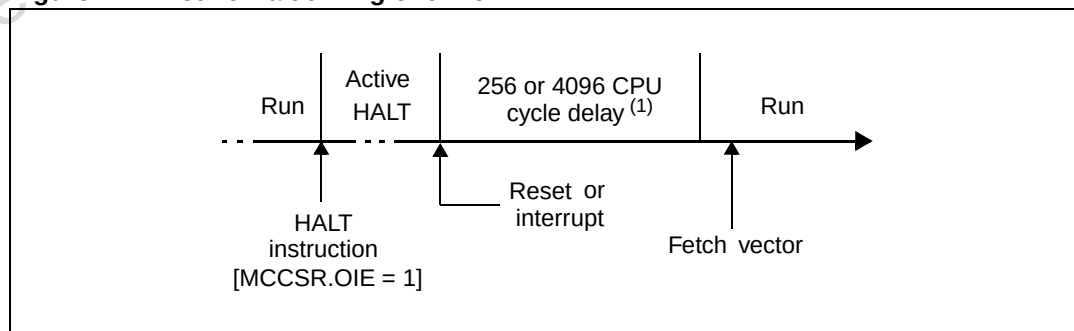
Figure 24. Active Halt timing overview
