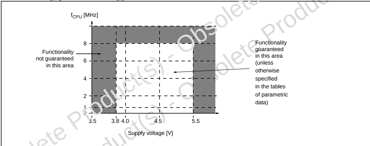
Figure 131. f_{\text{CPU}} max versus V_{\text{DD}}
