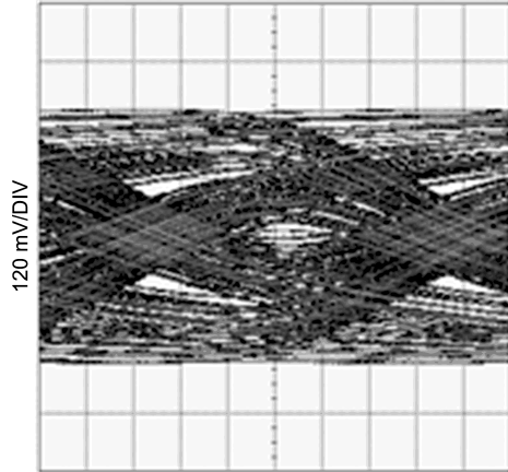
20 ps/DIV Figure 16.
