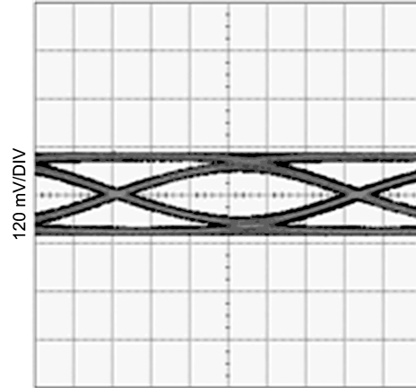
20 ps/DIV Figure 17.
