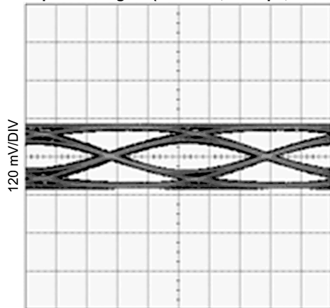
20 ps/DIV Figure 20.
