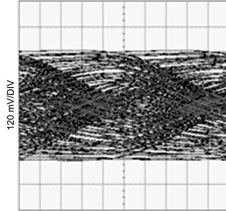
20 ps/DIV Figure 19.
