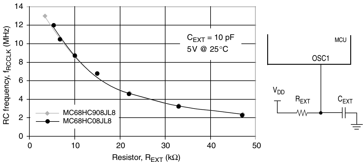
Figure 3. RC vs. Frequency (5V @ 25°C)
