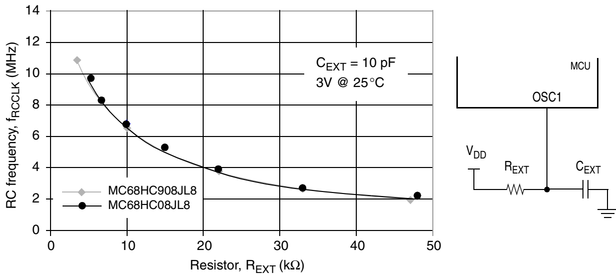
Figure 4. RC vs. Frequency (3V @ 25°C)
