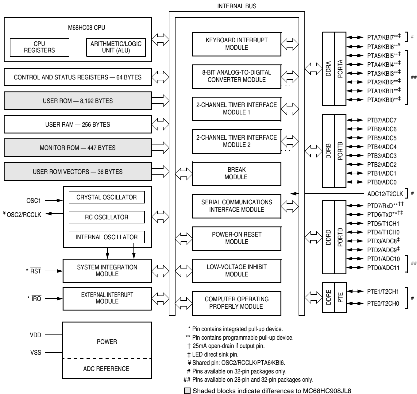
Figure 1. MC68HC08JL8 Block Diagram
