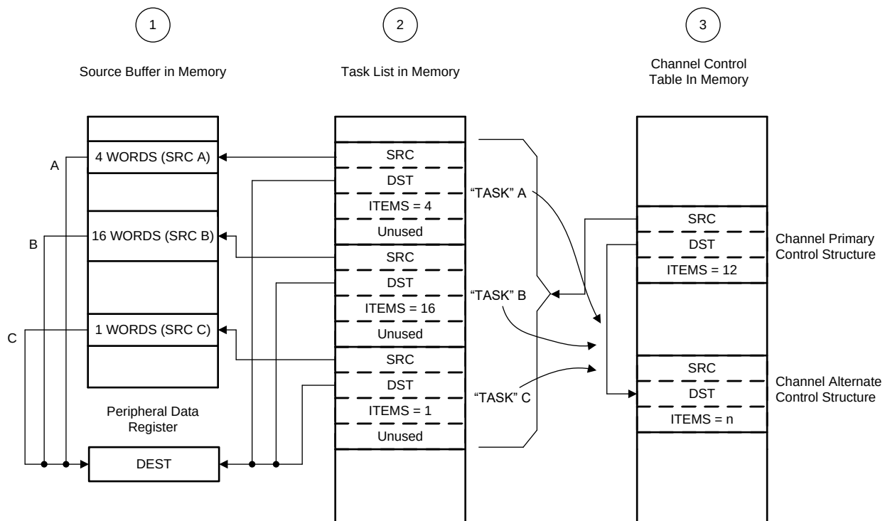
Figure 4-3. Peripheral Scatter-Gather Mode
