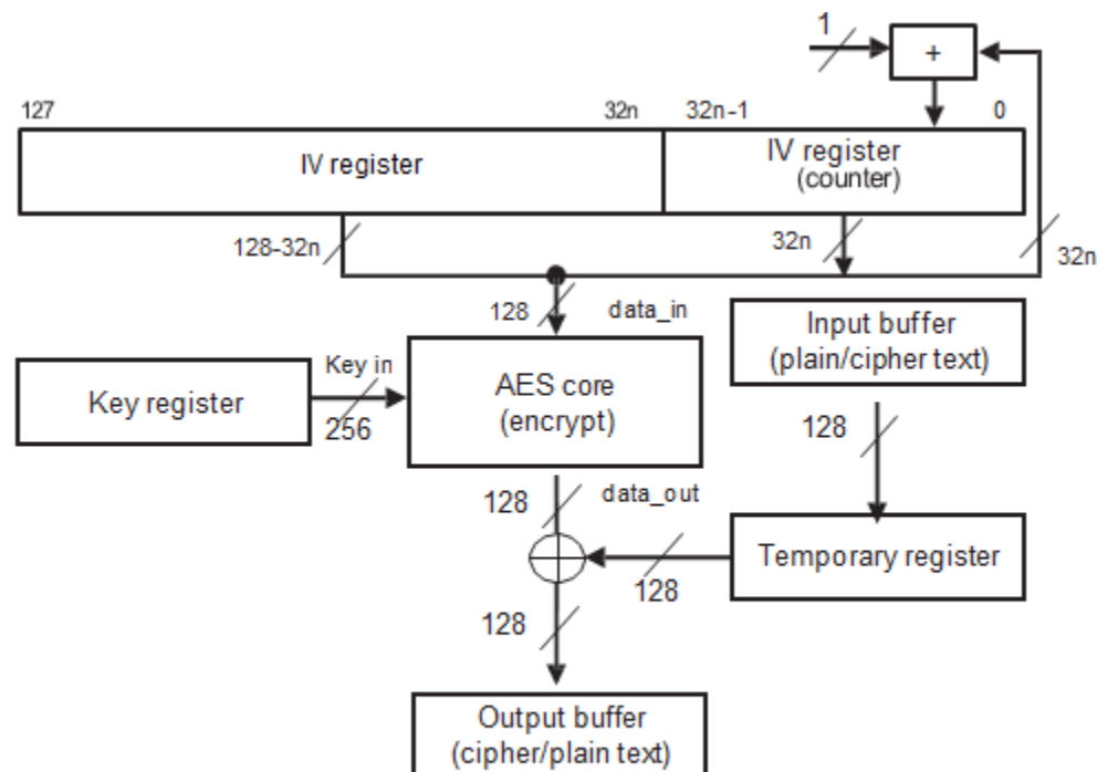
Figure 17-4. AES Encryption With CTR/ICM Mode
