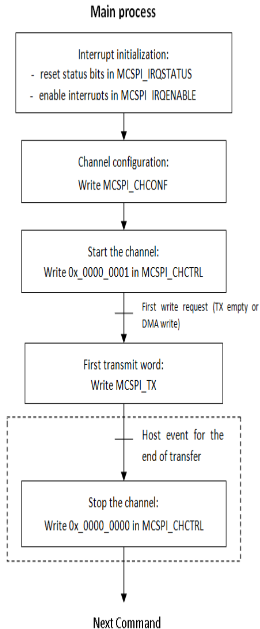
Figure 8-15. Flow Chart – Common Transfer Sequence
