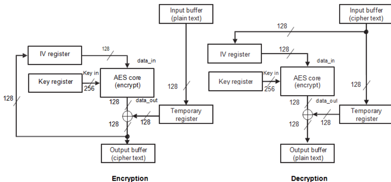
Figure 17-5. AES - CFB Feedback Mode
