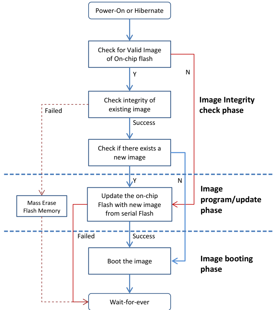
Figure 21-10. CC3235SF Boot Flow
