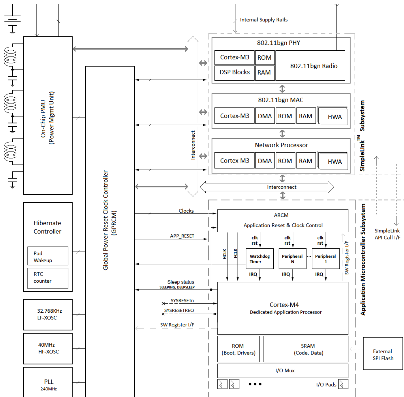
Figure 15-3. Power Management Control Architecture in CC32xx
