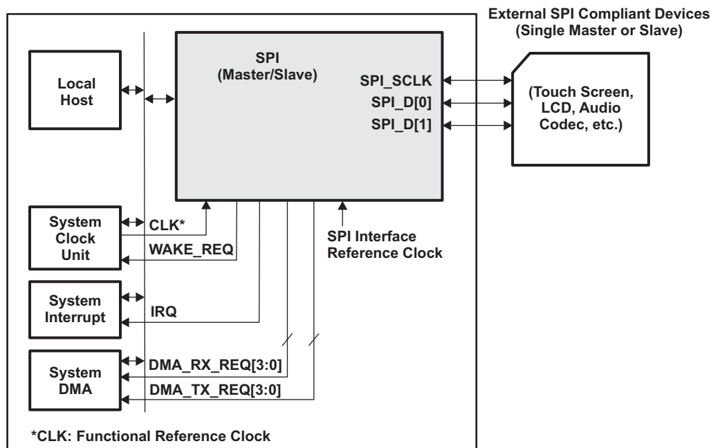
Figure 8-1. SPI Block Diagram
