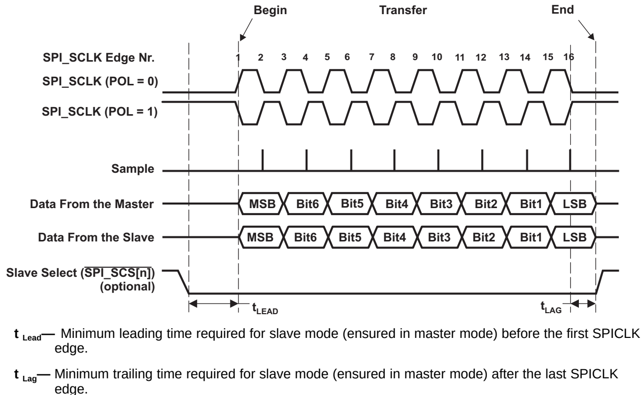
Figure 8-5. Full-Duplex Single Transfer Format With PHA = 1
