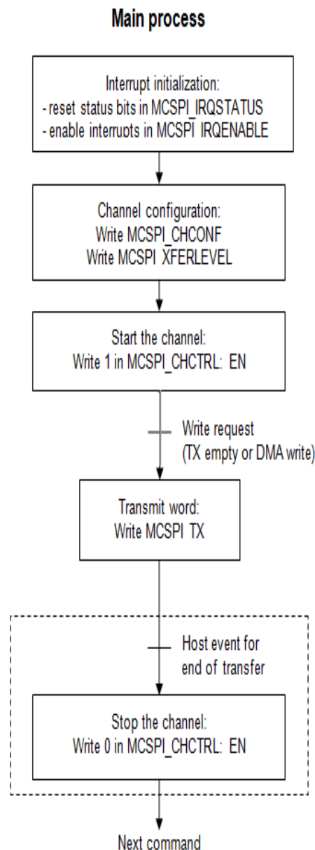
Figure 8-17. Flow Chart – FIFO Mode Common Sequence (Master)
