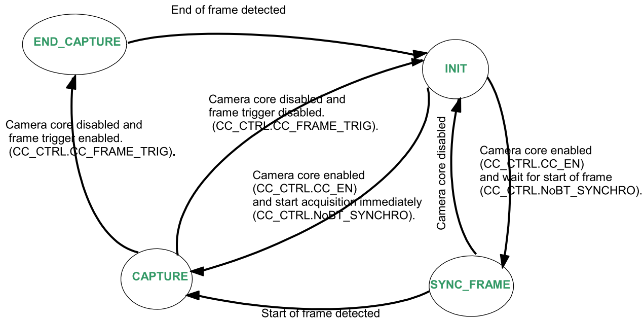
Figure 14-6. Parallel Camera Interface State Machine
