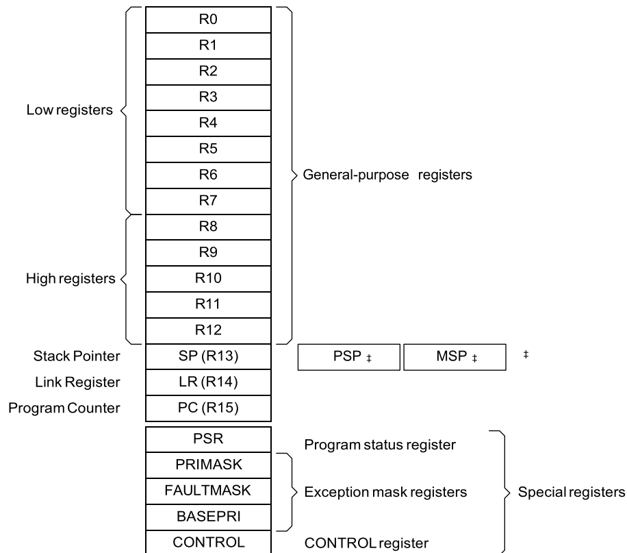
Figure 2-3. Cortex®-M4 Register Set
