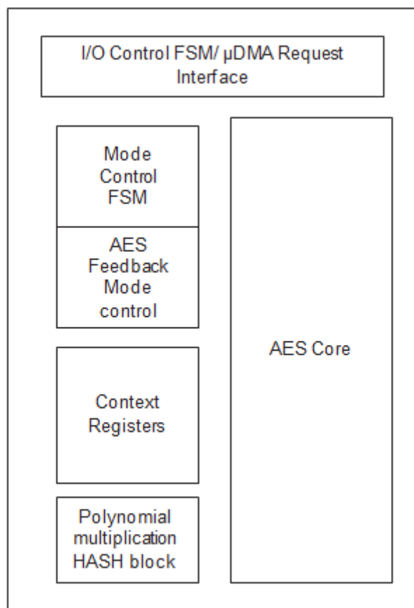
Figure 17-1. AES Block Diagram
