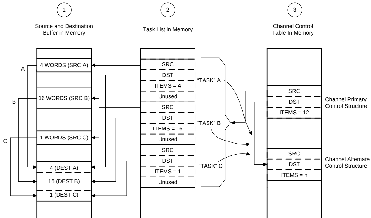
Figure 4-2. Memory Scatter-Gather Mode
