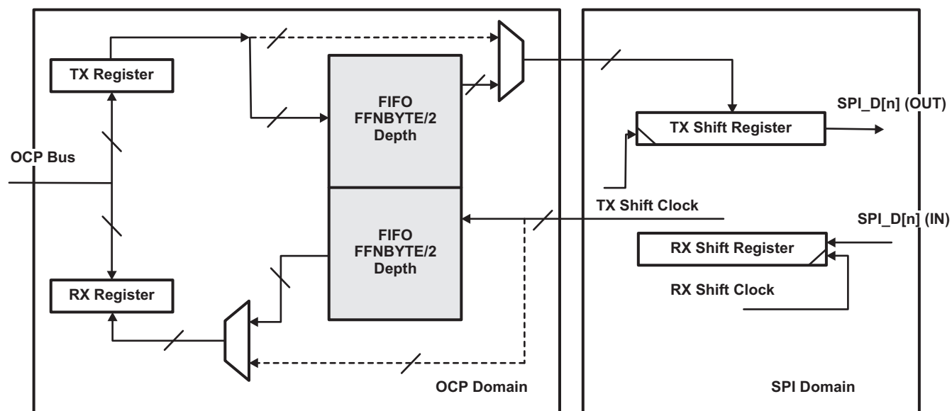
Figure 8-10. Transmit/Receive Mode With Both FIFO Directions Used
