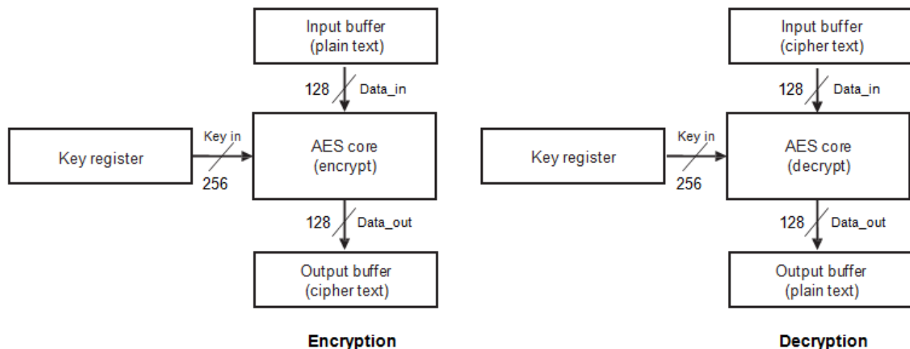
Figure 17-2. AES - ECB Feedback Mode
