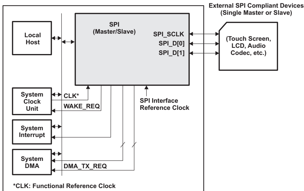
Figure 8-13. 3-Pin Mode System Overview
