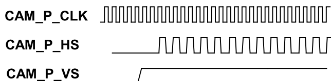
Figure 14-5. CAM_P_HS Toggles Between Pixels in Decimation
