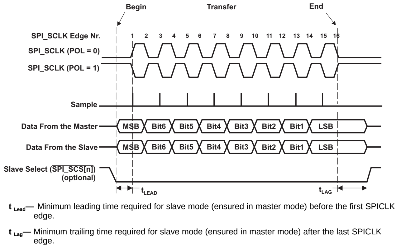
Figure 8-4. Full-Duplex Single Transfer Format With PHA = 0
