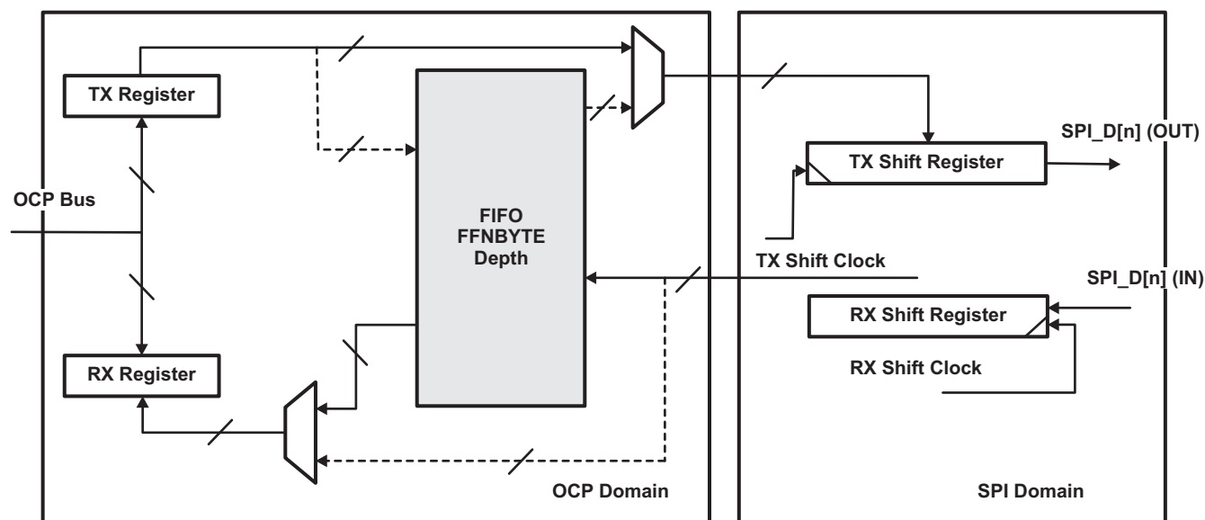
Figure 8-8. Transmit/Receive Mode With Only Receive FIFO Enabled
