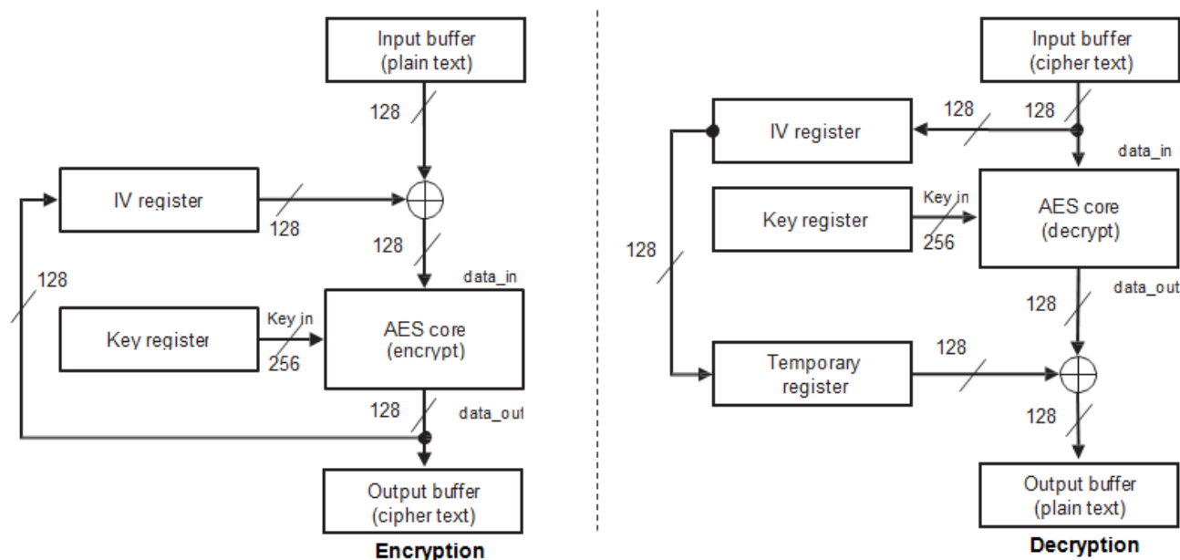
Figure 17-3. AES - CBC Feedback Mode
