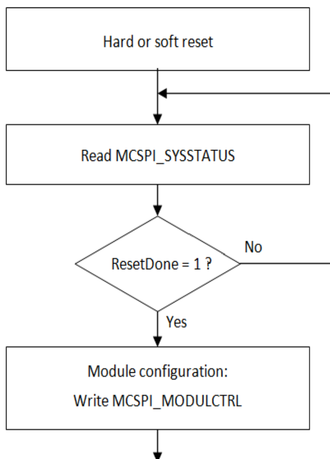
Figure 8-14. Flow Chart – Module Initialization
