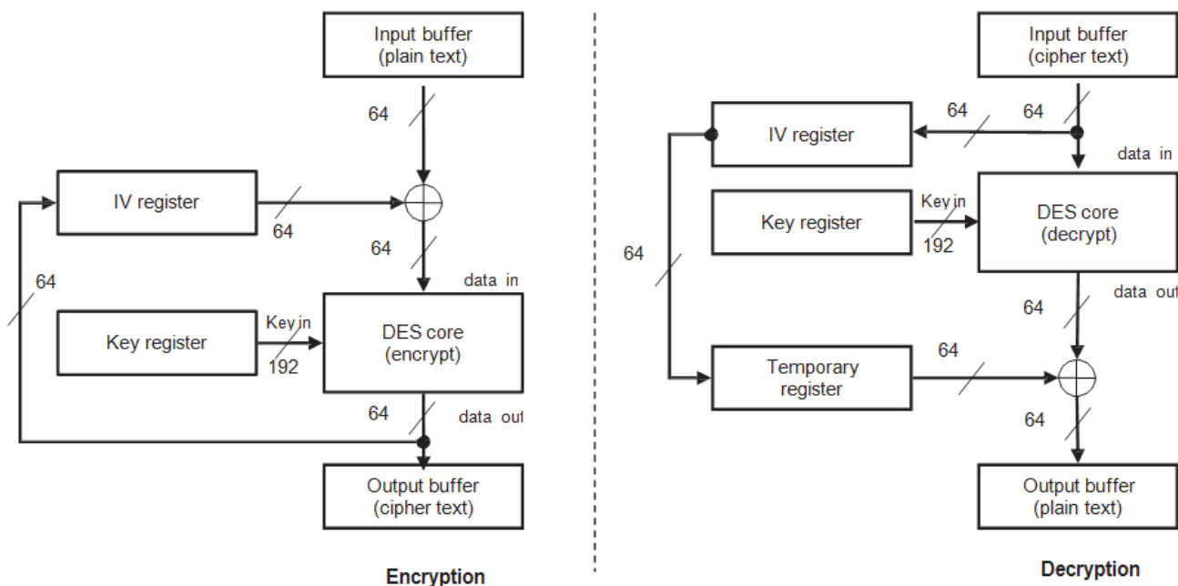
Figure 18-3. DES3DES – CBC Feedback Mode
