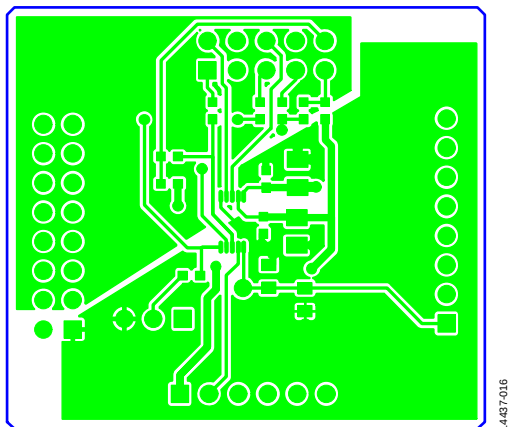
Figure 16. EVAL-AD5310RDBZ Daughter Board Top Side Routing
