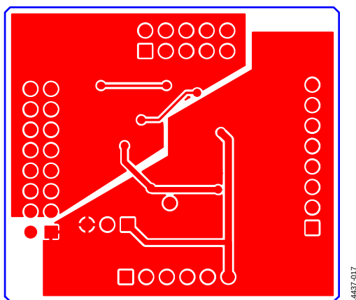
Figure 17. EVAL-AD5310RDBZ Daughter Board Bottom Side Routing
