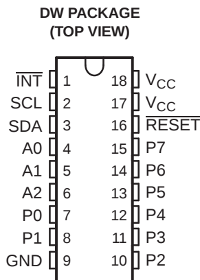
Pin Functions
