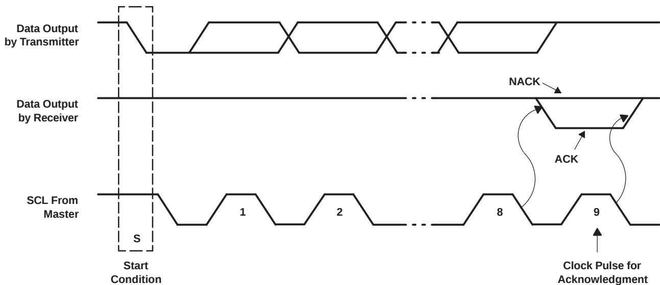
Figure 22. Acknowledgment On The I²C Bus
