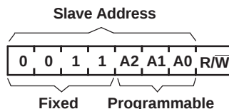
Figure 23. Pca6107 Address
