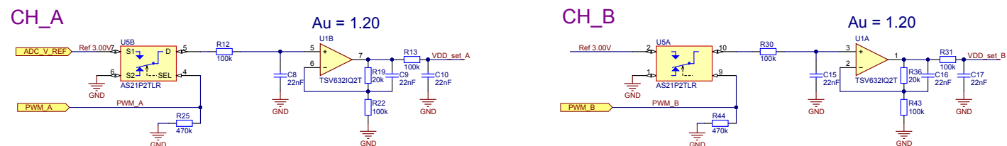
Dual channel Vdd control
