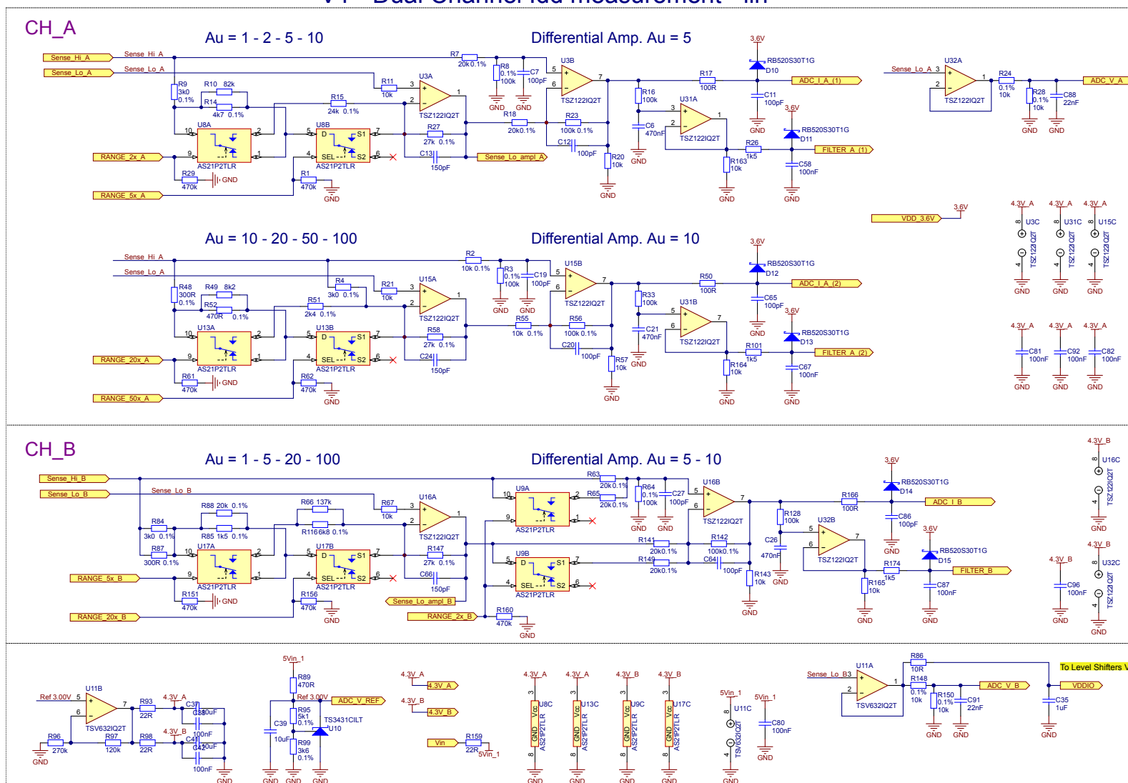
Figure 4. STEVAL-MKI109V3 circuit schematic (4 of 8)
