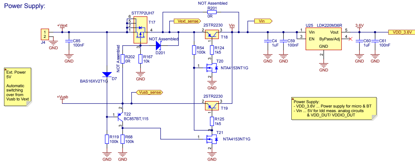
Figure 5. STEVAL-MKI109V3 circuit schematic (5 of 8)
