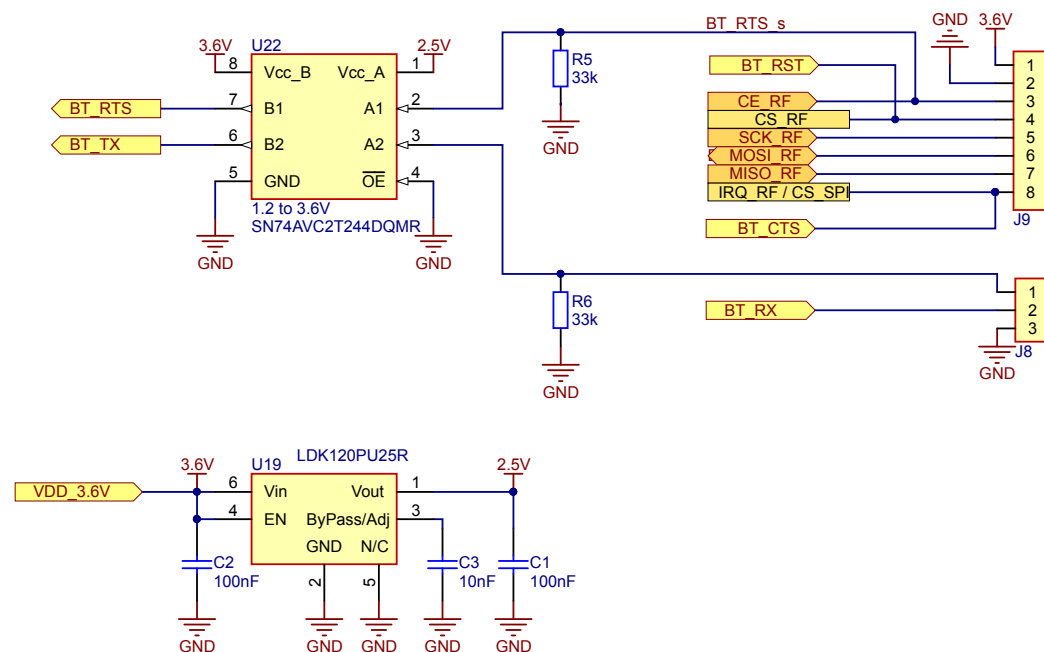
Bluetooth Module Connection:
