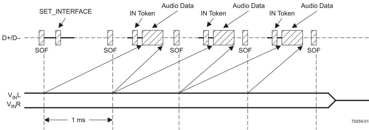
Figure 34. Record Sequence
