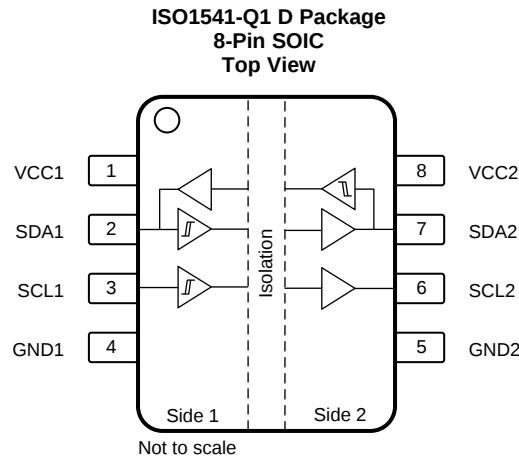
Pin Functions—ISO1541-Q1
