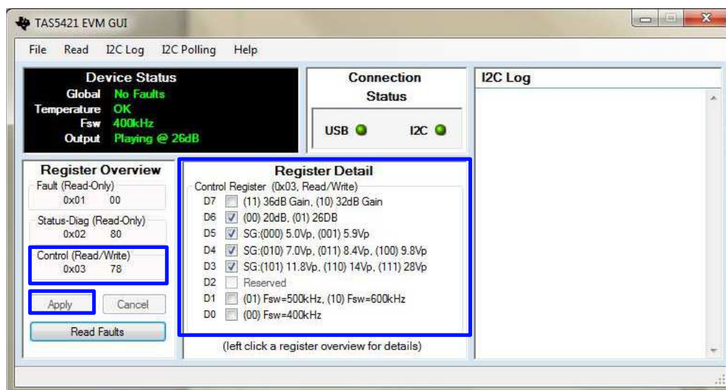
Figure 7. Control Register
