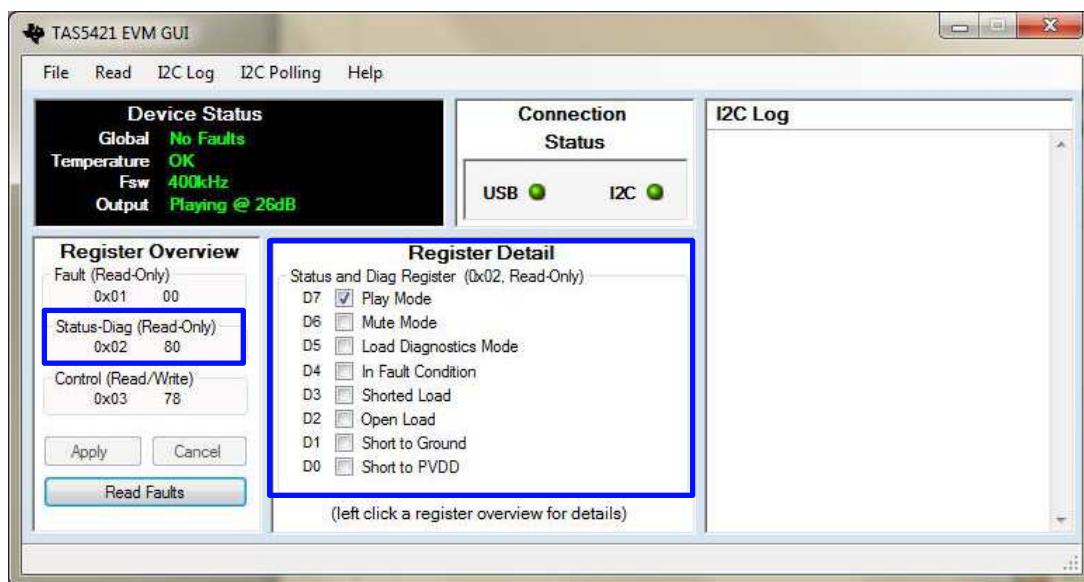
Figure 6. Status Register
