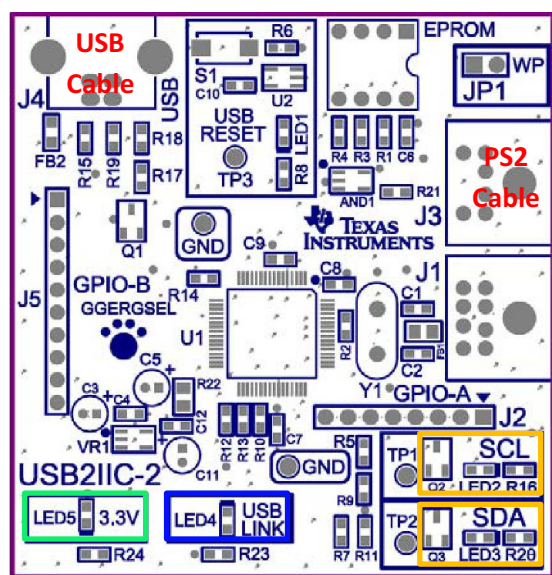
Figure 3. USB2IIC-2 Board
