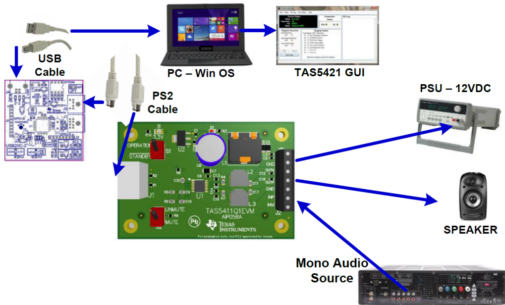
Figure 2. TAS5411EVM Connection
