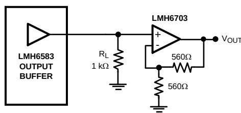
Figure 64. Buffered Output
