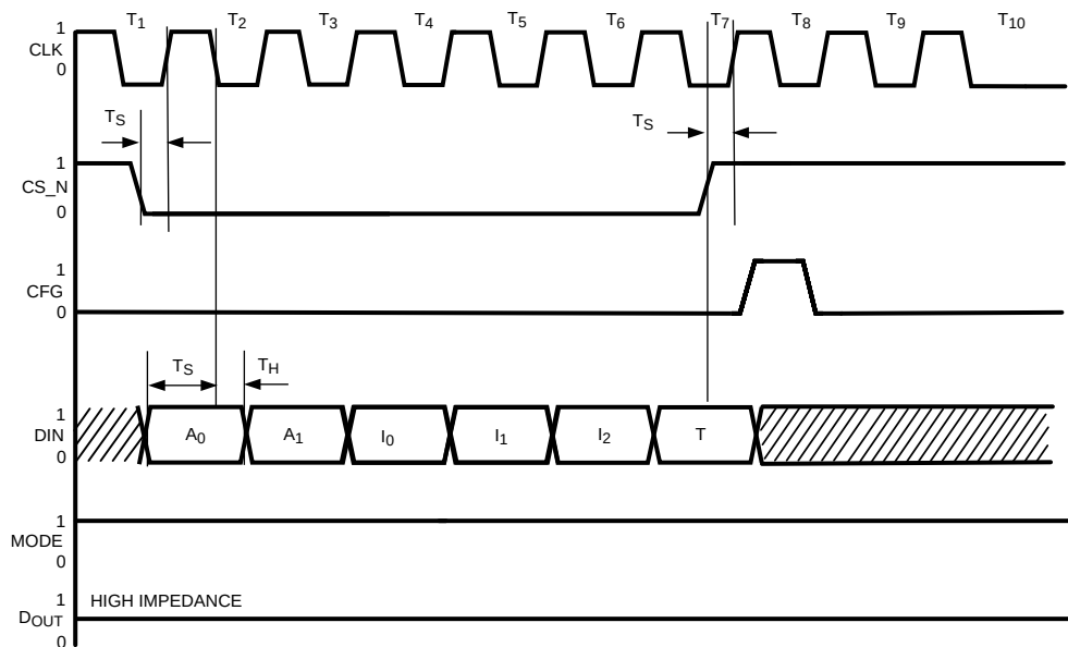
Figure 67. Timing Diagram for Addressed Mode
