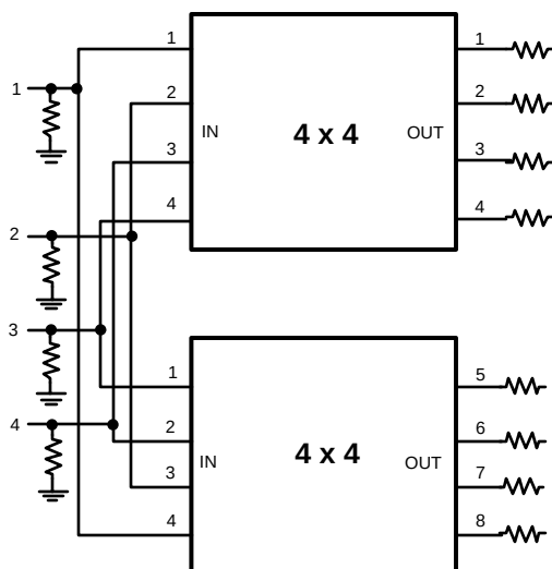
Figure 59. Output Expansion
