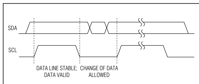
Figure 10. Bit Transfer
