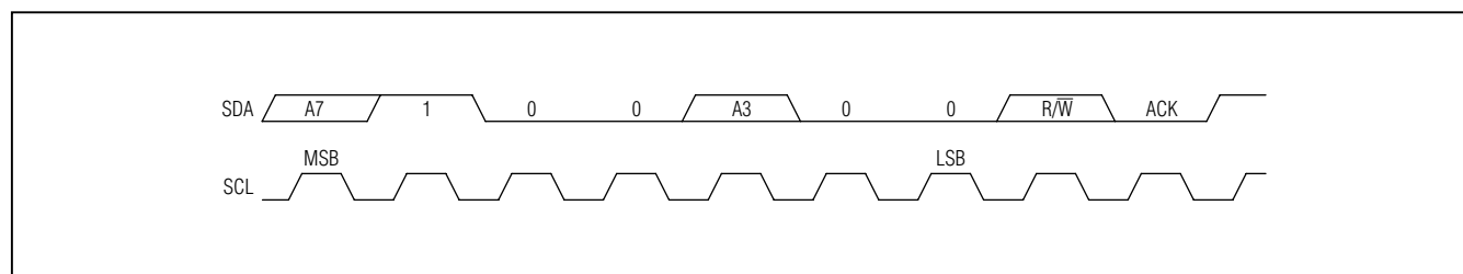
Figure 12. Slave Address
