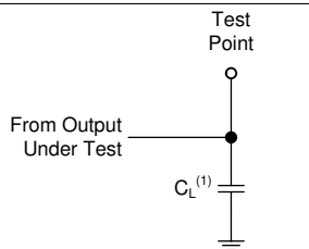
C_L = 50 \text{ pF} and includes probe and jig capacitance. Figure 3. Load Circuit
