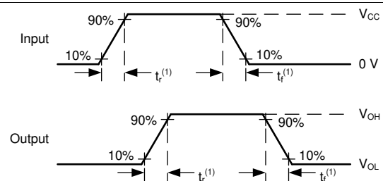
Figure 4. Voltage Waveforms Transition Times
