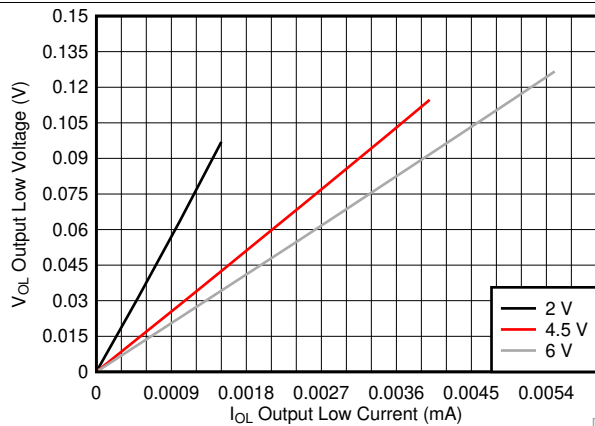
Figure 1. Output voltage versus output current in low state
