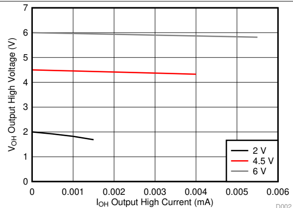
Figure 2. Output voltage versus output current in high state
