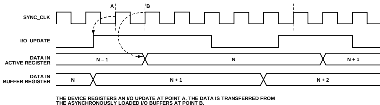
Figure 35. I/O Synchronization Timing Diagram
