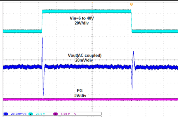
Figure 12. Line Transient Response, I_L = 10 \text{ mA} , 1 V/ \mu s
