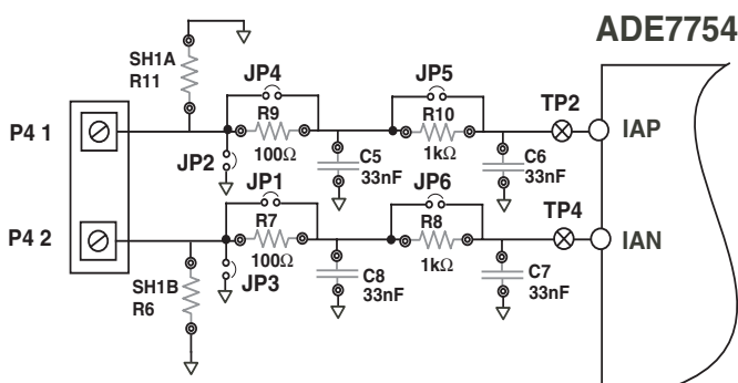
Figure 1 — Current Channel on the ADE7754 evaluation board
