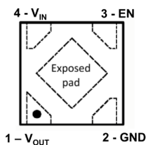
DFN4-1x1 (marking view)
