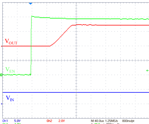
Figure 28. Enable transient ( I_{OUT} = 0 mA)
