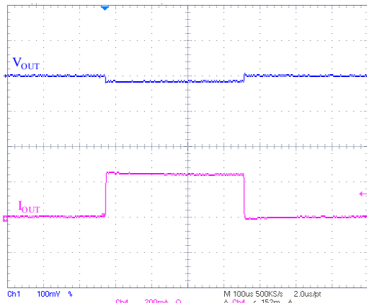
Figure 26. Load transient
