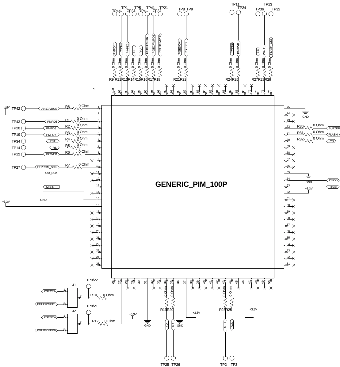
FIGURE 1: 100-PIN HEADER SCHEMATIC
