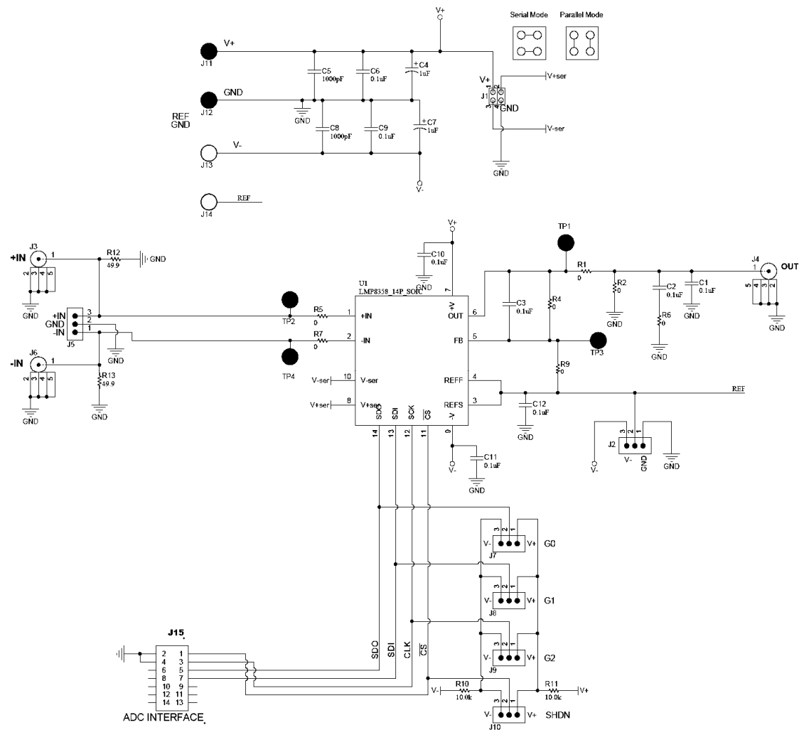
Figure 2. PCB Schematic
