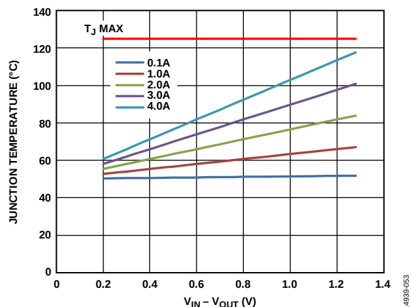
Figure 53. 1000 mm² of PCB Copper, T_B = 50^\circ\text{C} , LFCSP
