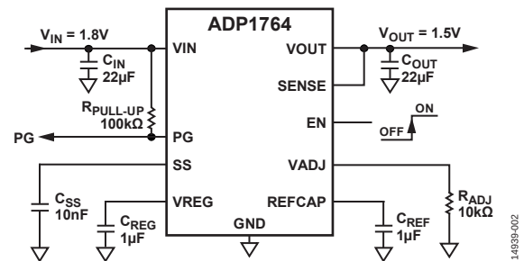
Figure 2. Adjustable Output Operation
