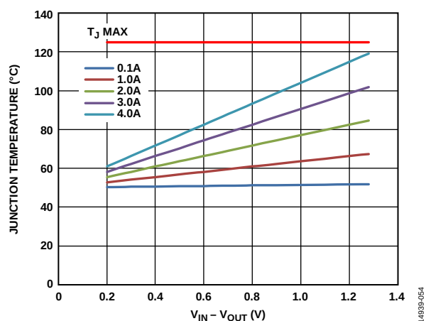
Figure 54. 500 mm² of PCB Copper, T_B = 50^\circ\text{C} , LFCSP
