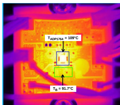
Figure 56. Thermal Image of the ADP1764 Evaluation Board at I_{LOAD} = 4\text{ A} , V_{IN} = 1.5\text{ V} , V_{OUT} = 1.3\text{ V} , T_B = 91.7^\circ\text{C}
