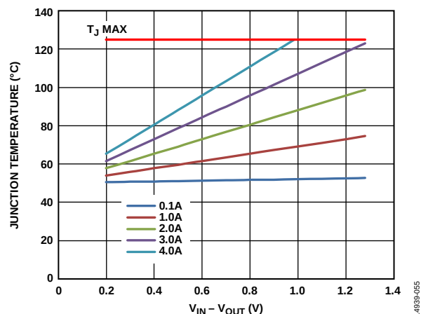
Figure 55. 100 mm² of PCB Copper, T_B = 50^\circ\text{C} , LFCSP
