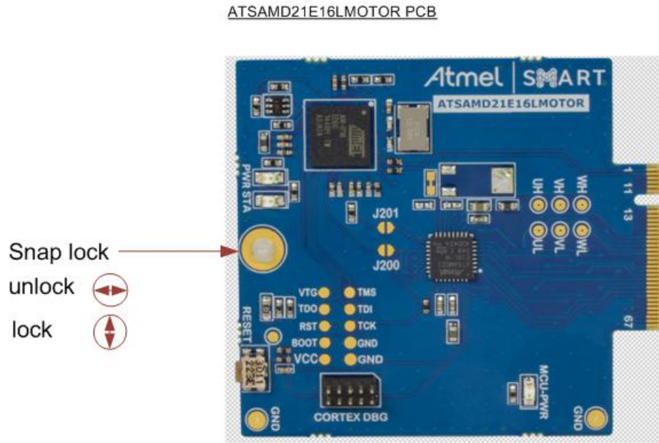
Figure 3-1. ATSAM21E16LMOTOR Kit Content
