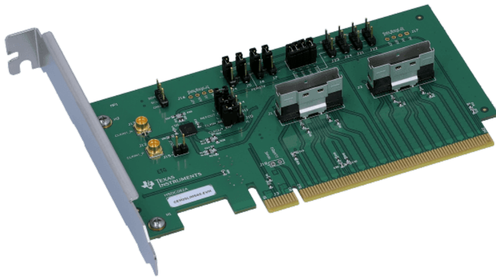
Figure 1. CEM2SLIMSAS-EVM - Top Side Photo
