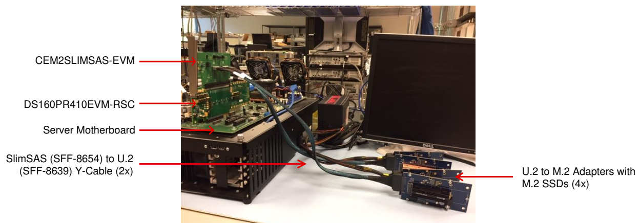
Figure 2. Example Test Setup
