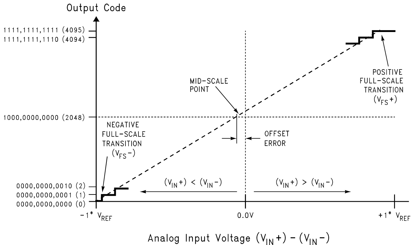
Figure 3. Transfer Characteristic
