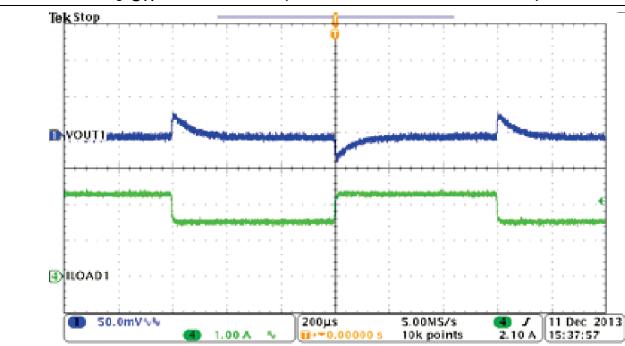
Figure 44. Buck1, Load Transient, 1.5 to 2.25 A SR = 0.25 A/ \mu\text{s}
