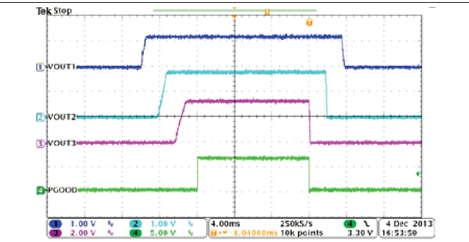
Figure 56. Automatic Power Sequencing, MODE = EN1 = EN2 = HIGH
