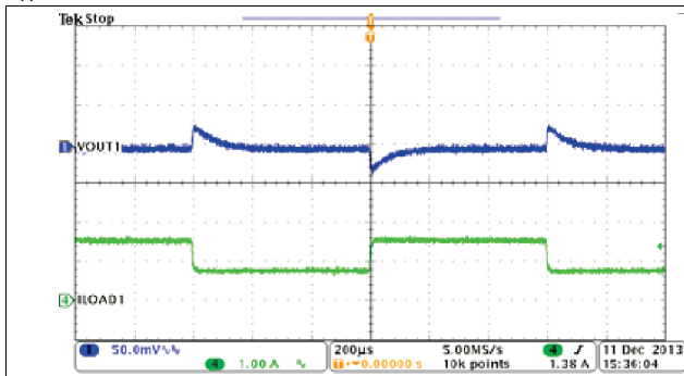
Figure 43. Buck1, Load Transient, 0.75 to 1.5 A SR = 0.25 A/ \mu\text{s}
