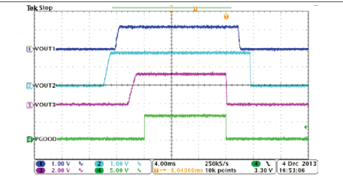
Figure 58. Automatic Power Sequencing, MODE = EN1 = HIGH, EN2 = LOW
