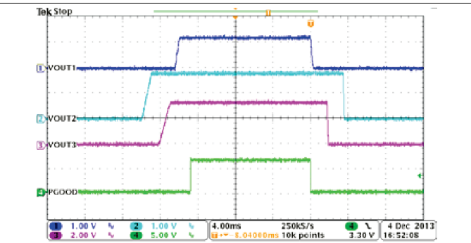
Figure 56. Automatic Power Sequencing, MODE = EN1 = EN2 = HIGH
