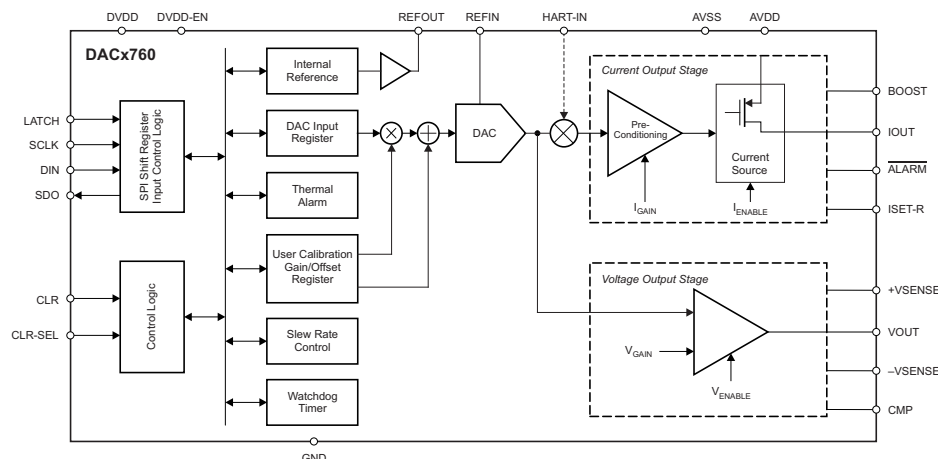
Block Diagram
