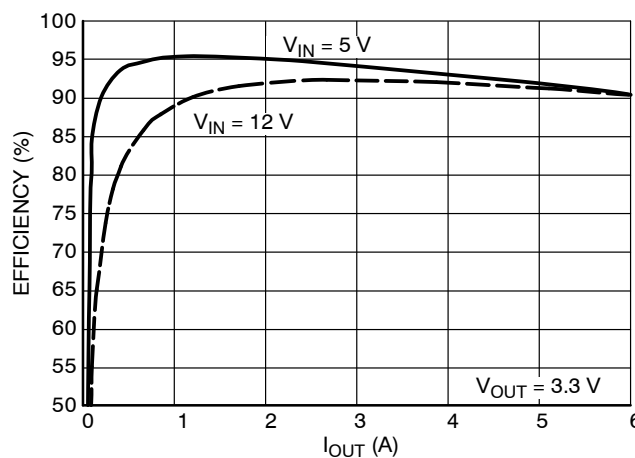
Figure 2. Efficiency
