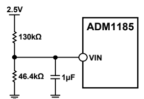
Figure 3. Introduction of Additional Delay
