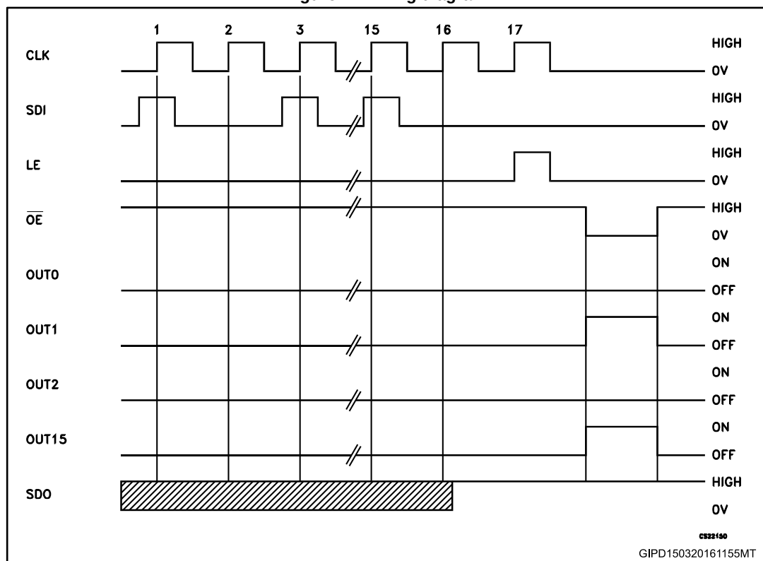
Figure 7: Timing diagram
