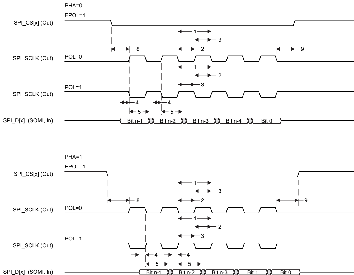
Figure 5-99. SPI Master Mode Receive Timing
