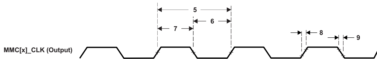
Figure 5-132. MMC[x]_CLK Timing
