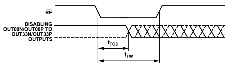
Figure 6. Asynchronous Reset
